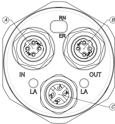
IN - OUT M12 4P Female D-coded connector connection
