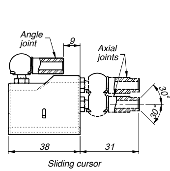
Sliding cursor, axial joint angle
